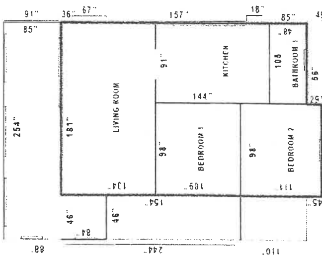
FIRST FLOOR 266"
